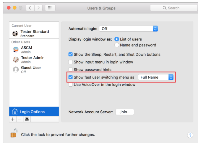
Figure 8. Login Options
