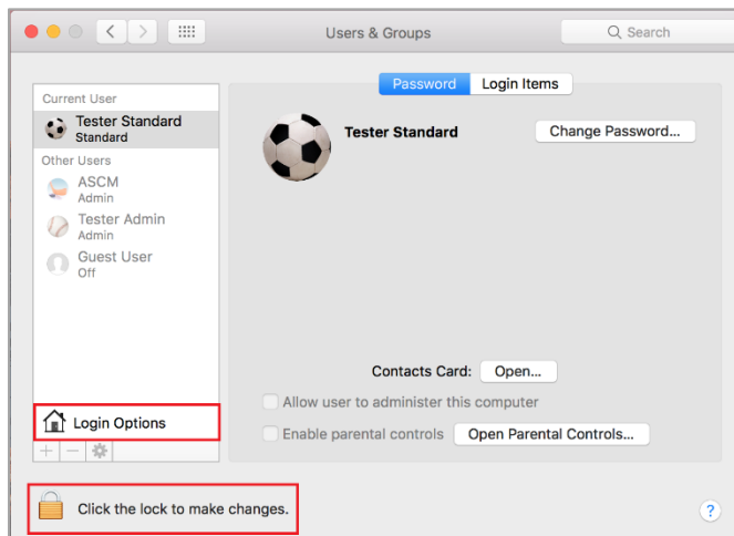
Figure 7. Users & Groups
