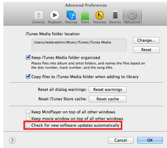
Figure 3. Advanced Preferences
