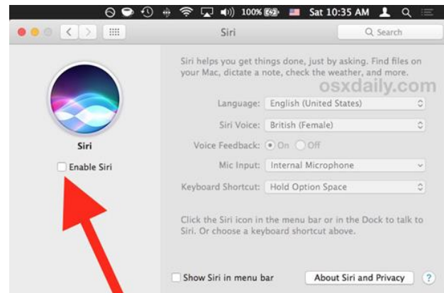
Figure 5. Siri
